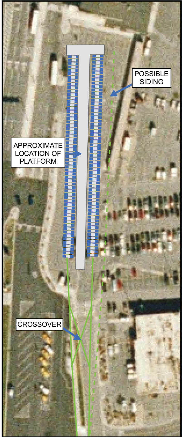
Source: SLCD, 2008 LRT Alignment Draft Report, Section 3.1, North of the Surplus Canal, Figure 5, Traction Power Substation #1, Figure 6, Interim Station, and Figure 7, Alignment Along 3700 W (June 2008).
